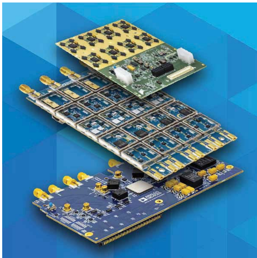
1. Analog Devices' X-Band Phased Array Platform features high-speed mixed-signal ICs assembled on three PCBs and works with a fourth controller PCB for extensive phased-array beamforming experimentation.
