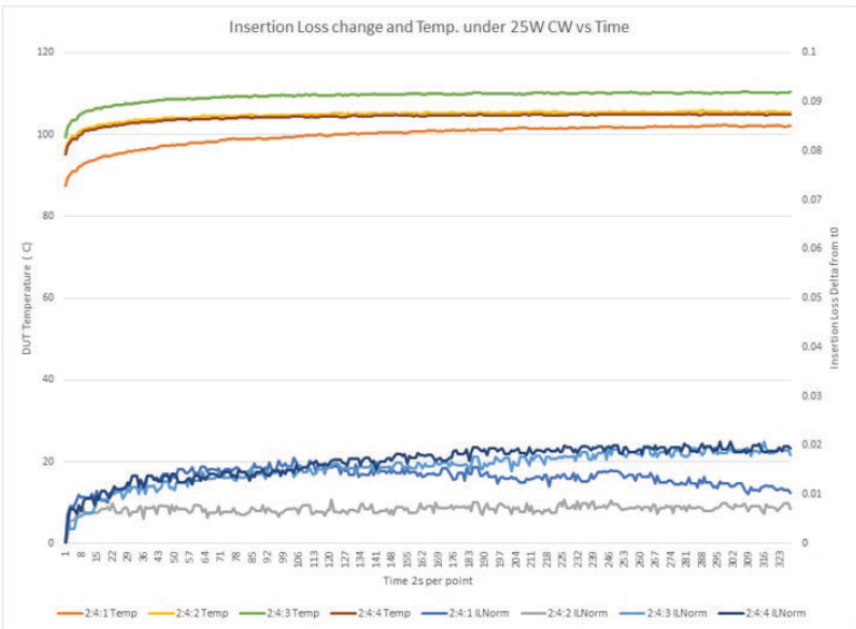
Typical variation of IL and package temp over time, while subjected to 25W CW at +85C
