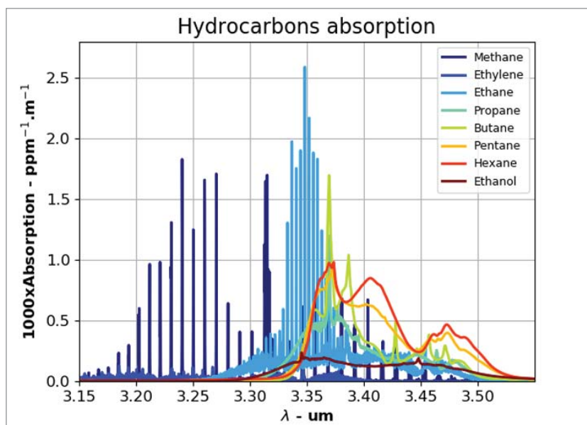
1. Shown are absorption rays of CH 4 and other gases, illustrating how sensors designed for this bandwidth also are sensitive to many other gases.
