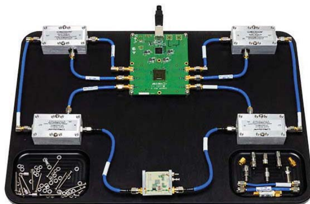
3. A microwave transceiver kit developed by Mini-Circuits includes a first lesson on how to assemble its components into a two-port VNA with a frequency range of 100 MHz to 6 GHz.
