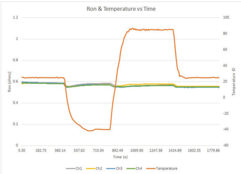
Typical variation of on resistance over temperature from -40C to +85C
